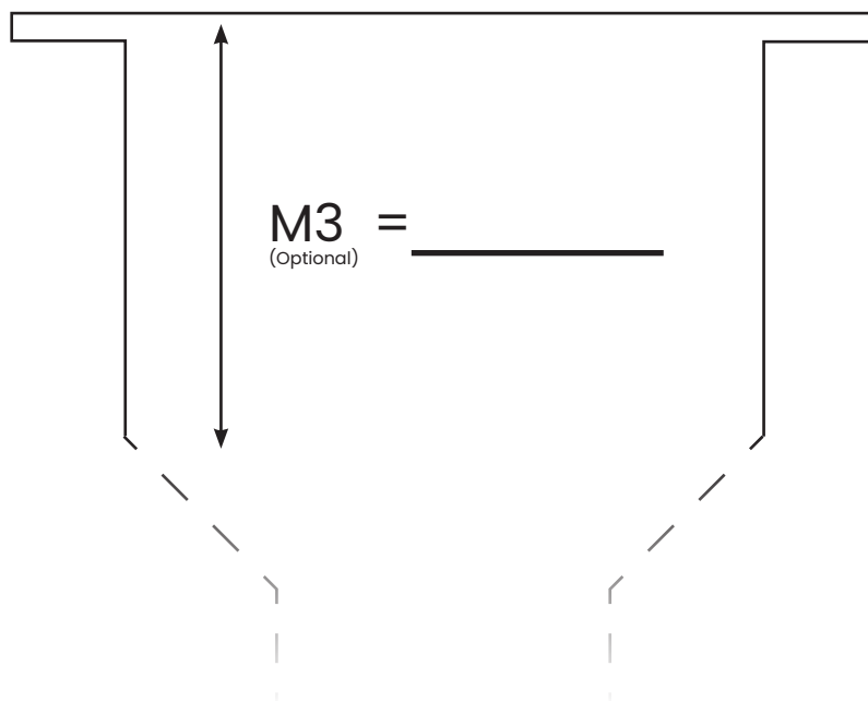
Profile View of Hawse Pipe
